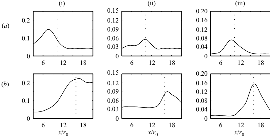
FIGURE 8. Case M_{40}/axis . Axial variation of peak correlation between pressure at M_{40} and flow quantities at x/r_0 along the jet axis. Peaks of (i) -Cup , (ii) Cuup , (iii) C|\omega|p , for (a) LESm09hre, (b) LESm09re1700. The dotted lines show the end of the potential core.
